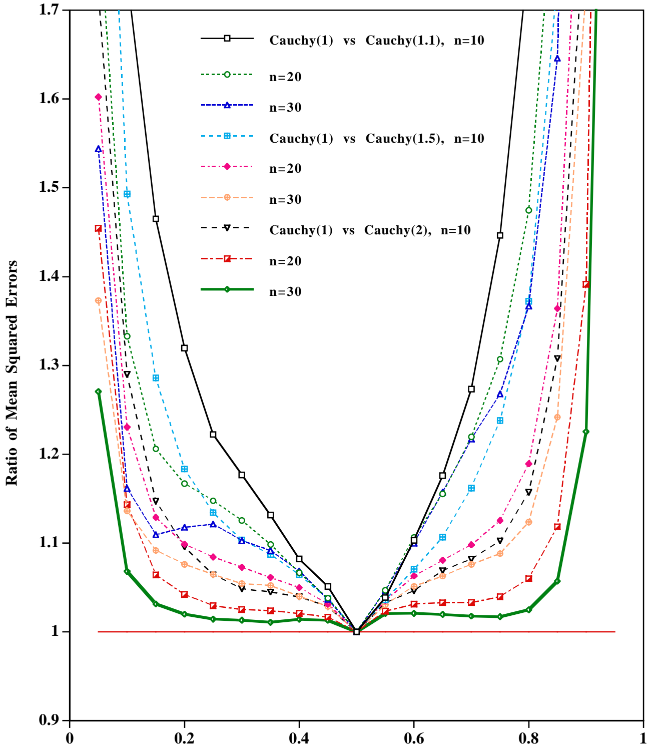
Figure 2.- Ratios of Mean Squared Errors (MSE) of the Kaplan-Meier to the constrained estimator in the one sample, censored, Cauchy case. The MSEs are evaluated at 19 quantiles of the underlying distribution.
