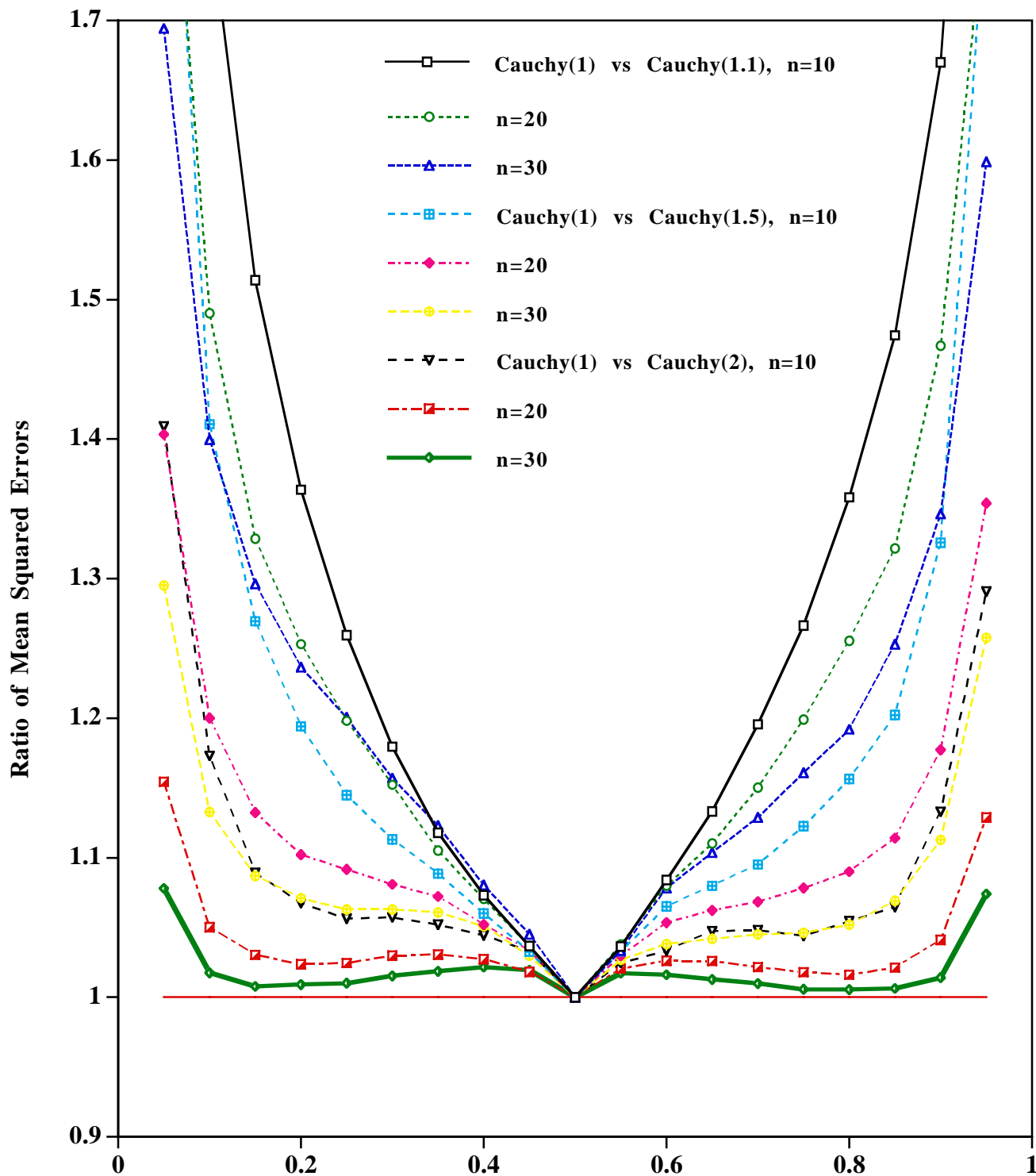
Figure 1.- Ratios of Mean Squared Errors (MSE) of the Empirical to the constrained estimator in the one sample uncensored Cauchy case. The MSEs are evaluated at 19 quantiles of the underlying distribution.
