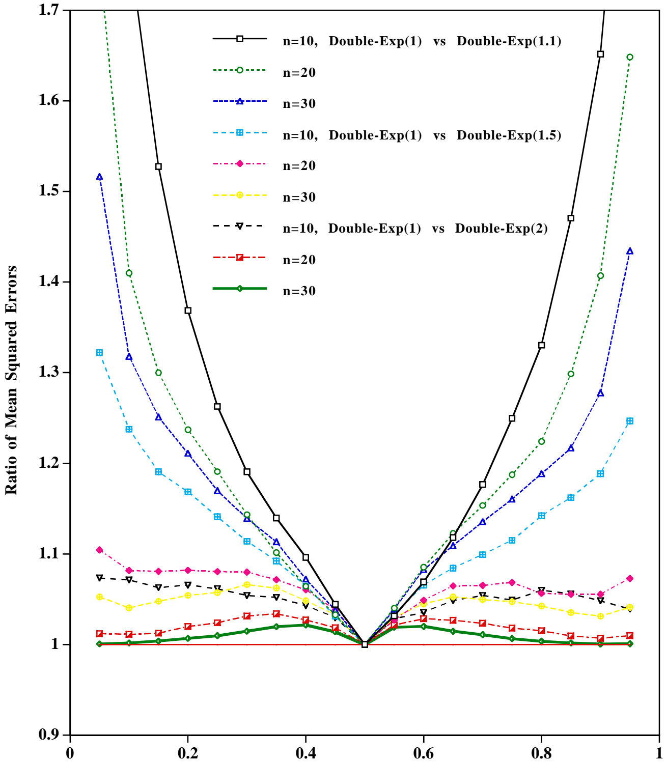
Figure 5.- Ratios of Mean Squared Errors (MSE) of the Empirical to the constrained estimator in the one sample, Double-Exponential case. The MSEs are evaluated at 19 quantiles of the underlying distribution.
