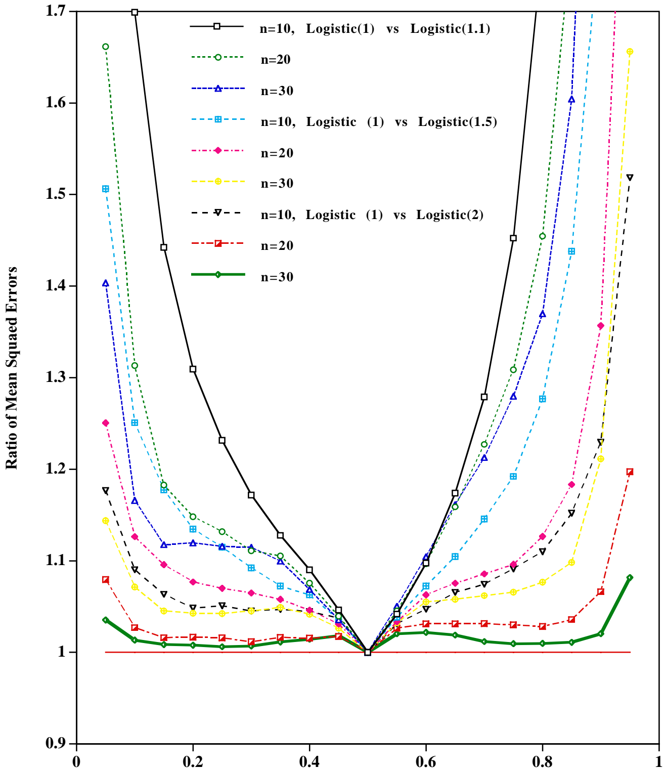
Figure 4.- Ratios of Mean Squared errors (MSE) of the Kaplan-Meier to the constrained estimator in the one sample, censored, Logistic case. The MSEs are evaluated at 19 quantiles of the underlying distribution
