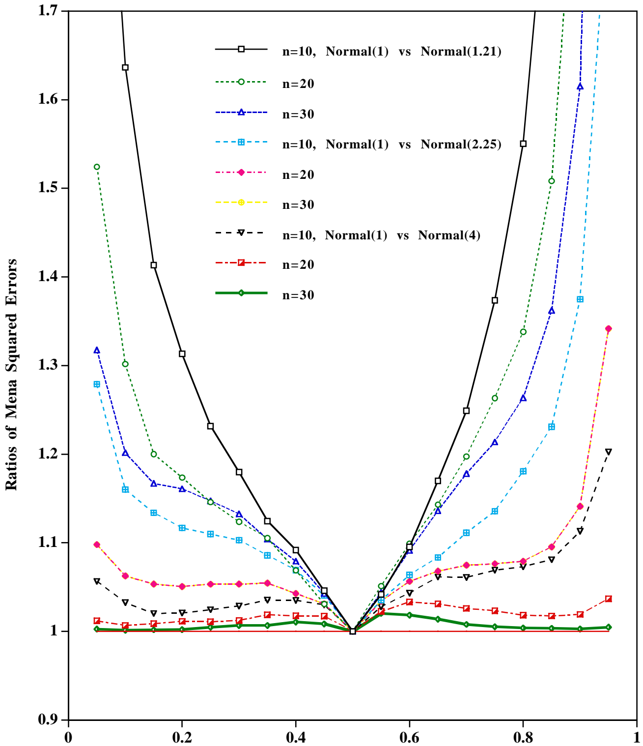
Figure 6.- Ratios of Mean Squared Errors (MSE) of the Kaplan-Meier to the constrained estimator in the one sample, censored, Normal case. The MSEs are evaluated at 19 quantiles of the underlying distribution.
