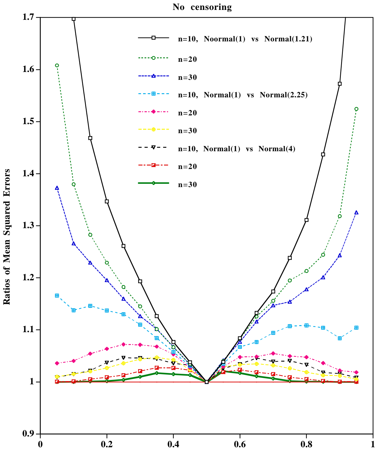
Figure 7.- Ratios of Mean Squared Errors (MSE) of the Empirical to the constrained estimator in the one sample uncensored Normal case. The MSEs are evaluated at 19 quantiles of the underlying distribution.
