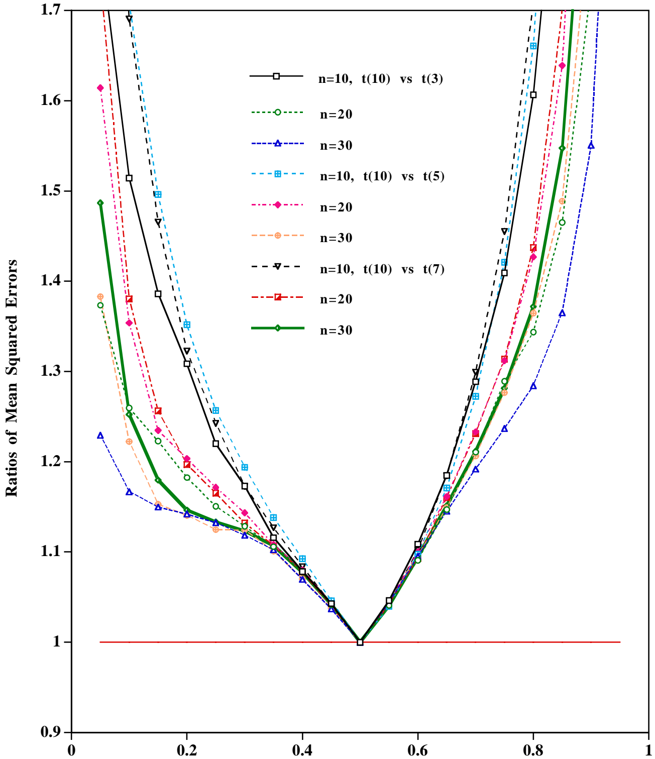
Figure 8.- Ratios of Mean Squared Errors (MSE) of the Kaplan-Meier to the constrained estimator in the one sample censored t distribution case. The MSEs are evaluated at 19 quantiles of the underlying distribution.
