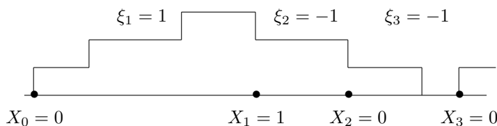
Figure 6.1: Realization of the M/G/1 queue.
