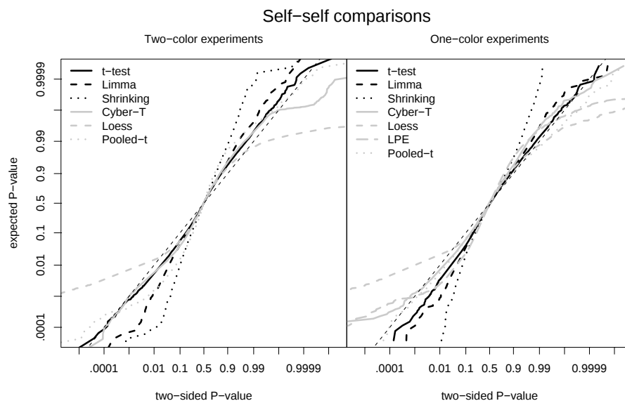
Figure 1.1 Performance of the various approaches to significance testing using an explicit reference distribution for small microarray experiments for the combined two-color and one-color self-versus-self experiments. For unbiased methods the curves should follow the identity line.
