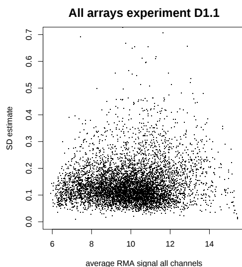
Figure 1.6 Relation between the residual standard deviation and the average RMA normalized expression for one of the one-color experiments.
