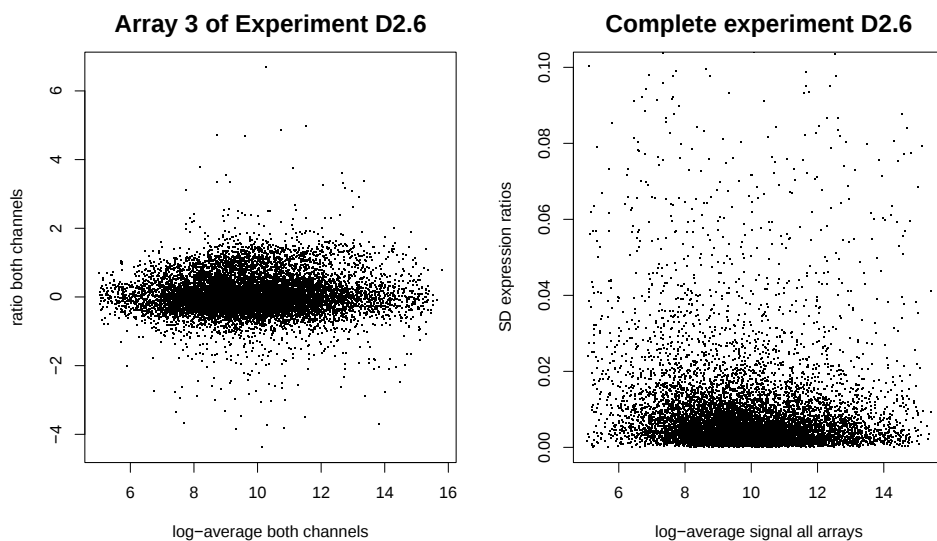
Figure 1.5 Relation between log expression ratio and average log expression for one normalized two-color array, and the standard deviation of log expression ratios with the average log expression ratio for all arrays from that experiment.
