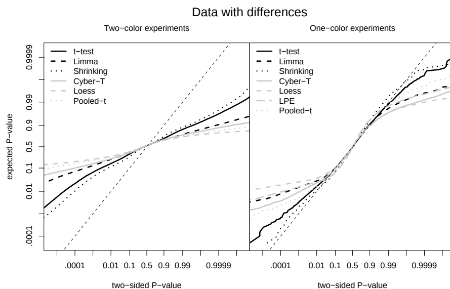
Figure 1.2 Performance of the various approaches to significance testing using an explicit reference distribution for small microarray experiments for the combined two-color and one-color experiments that involve different samples. More horizontal curves correspond to more powerful methods.
