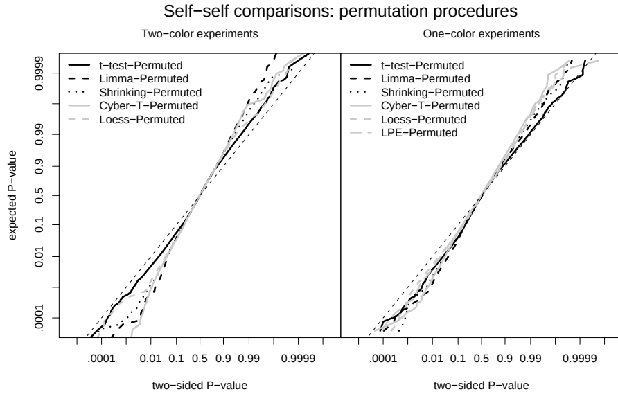
Figure 1.3 Performance of the various approaches to significance testing using a permutation approach rather than a reference distribution for small microarray experiments for the combined two-color and one-color self-versus-self experiments. For unbiased methods the curves should follow the identity line.
