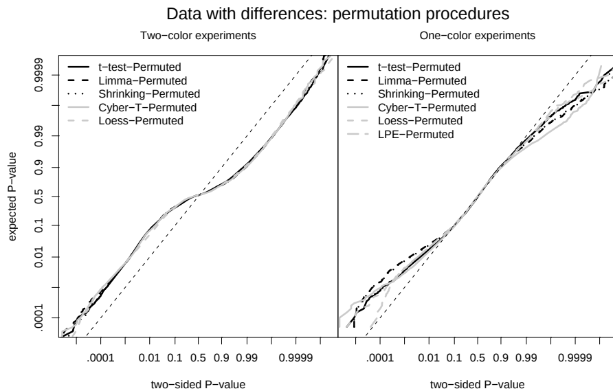
Figure 1.4 Performance of the various approaches to significance testing using a permutation approach for small microarray experiments for the combined two-color and one-color experiments that involve different samples. More horizontal curves correspond to more powerful methods.
