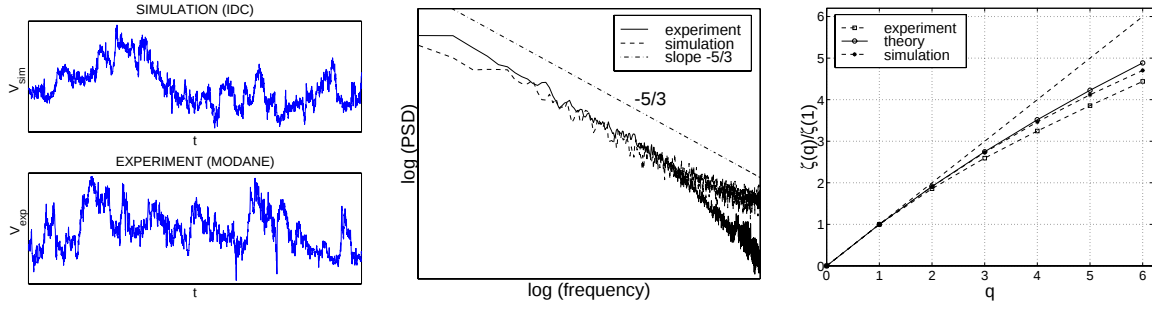
Fig. 4. Comparison between an IDC random walk following She-Lévy model and an experimental signal (Modane, Re \sim 2500 ): samples of velocity signals (left), power density spectra (middle), relative scaling exponents (right).
