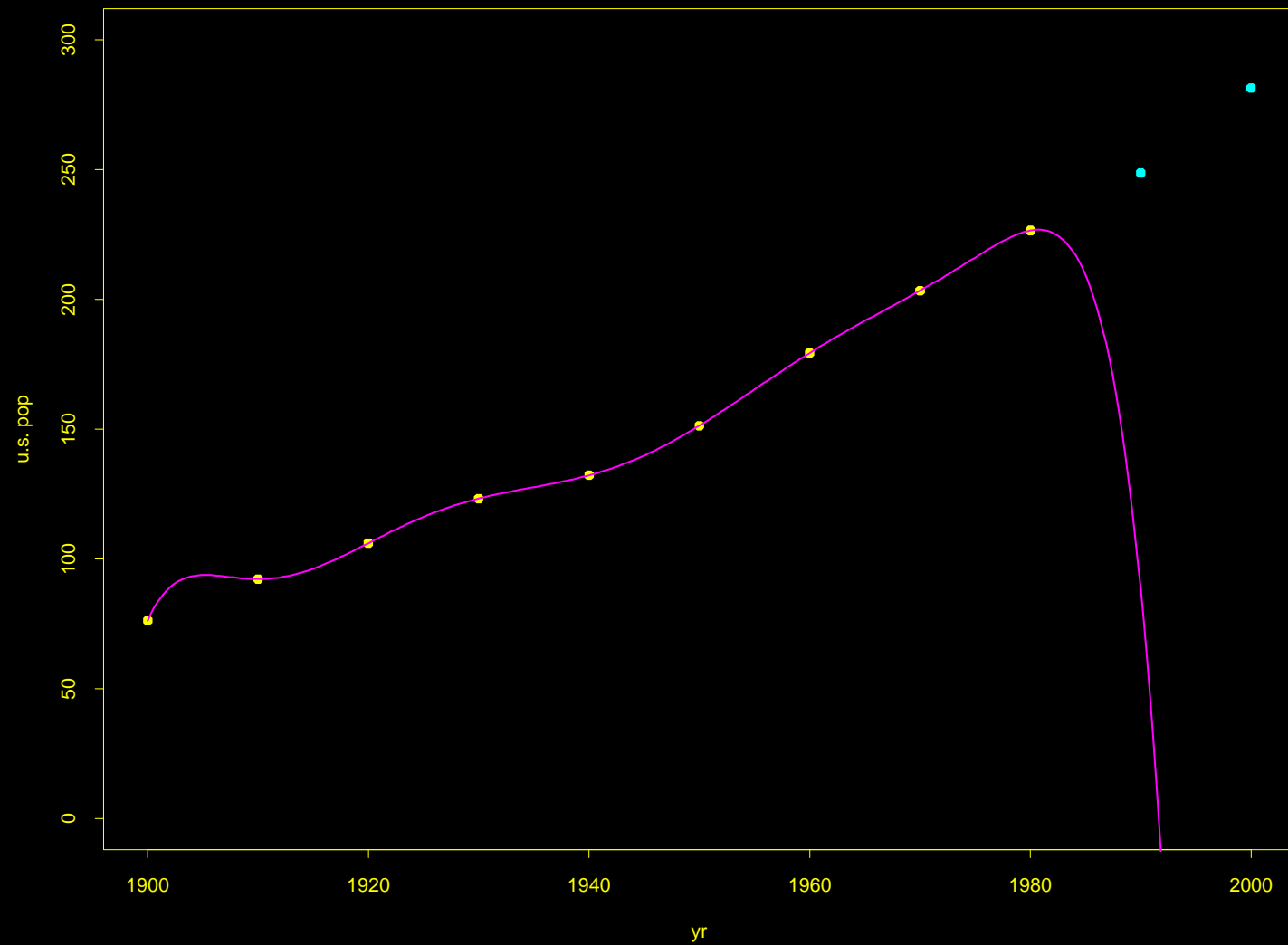
polynomial order 8
