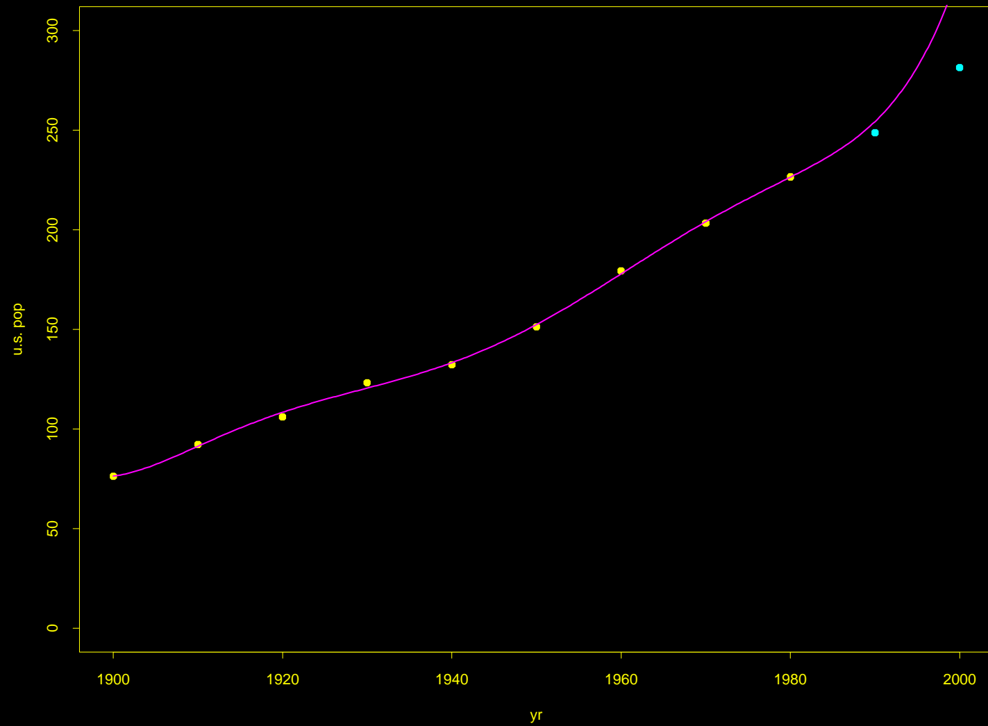
polynomial order 6
