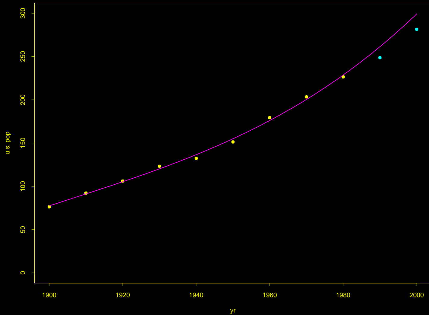
polynomial order 3
