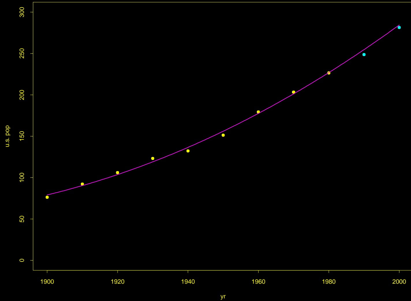
polynomial order 2
