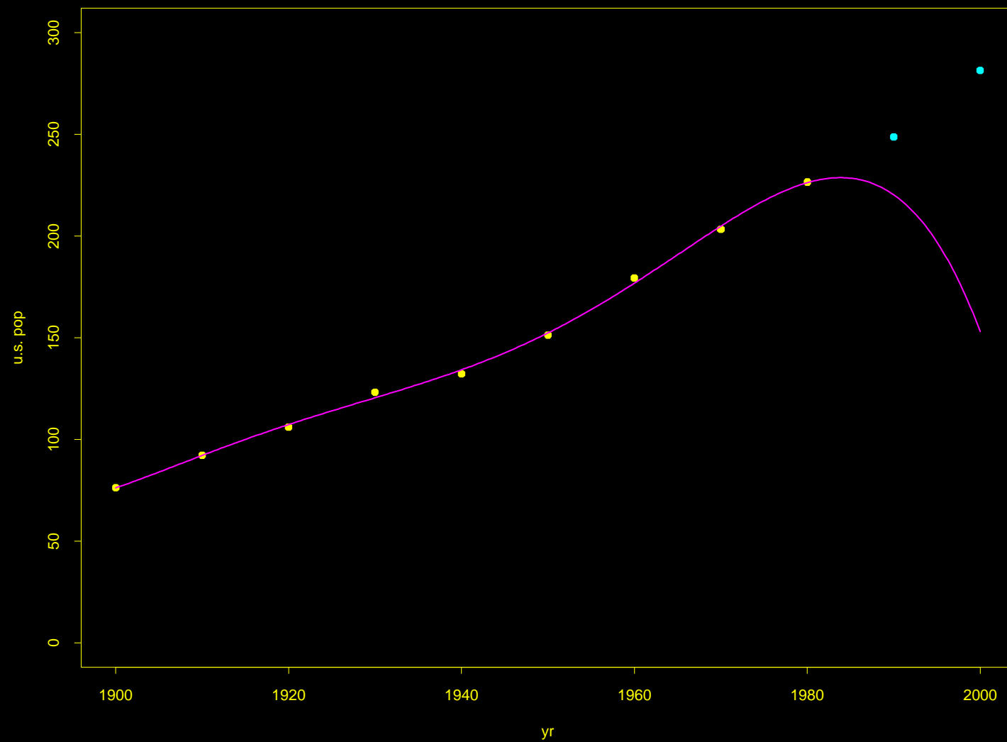
polynomial order 5
