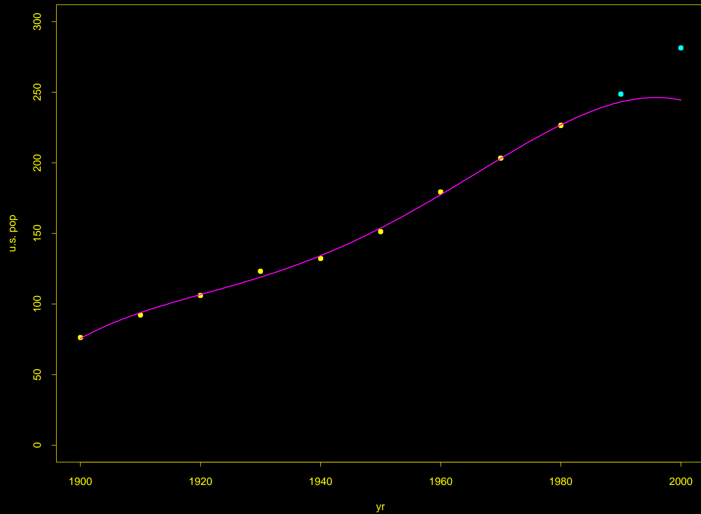
polynomial order 4
