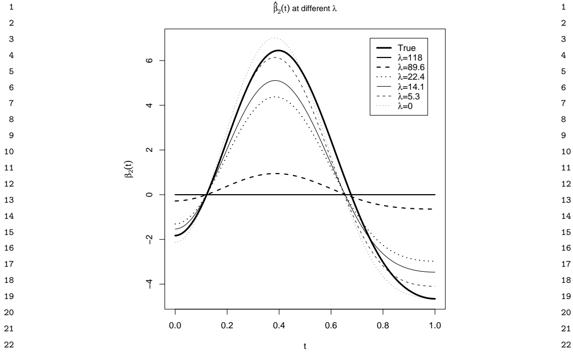
FIG 4. Estimated coefficient function \hat{\beta}_2(t) at 6 selected \lambda values and the true \beta_2(t) .
