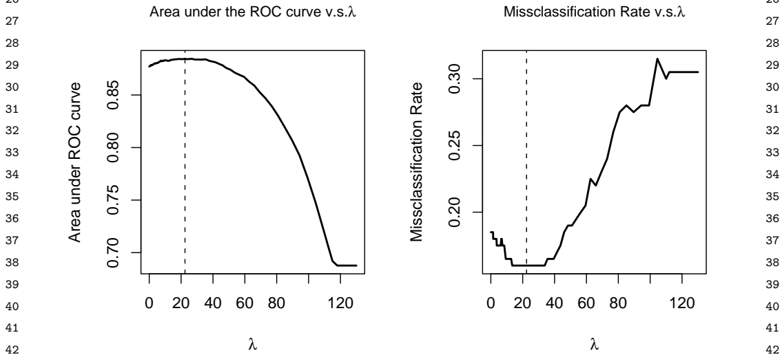
FIG 5. Prediction results at different \lambda values.
