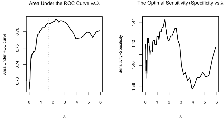
FIG 7. Prediction results at different \lambda values.
