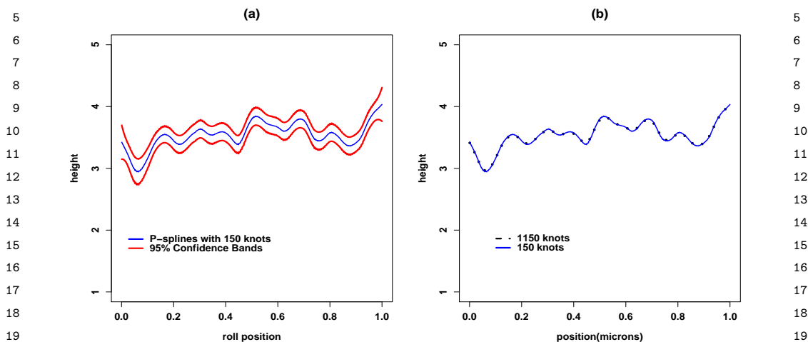
21 FIG 3. Figure (a) shows the P-spline estimator with 150 knots for the roller height with its 22 respective 95% confidence bands. The corresponding figure for the P-spline estimator with 1150 23 knots looks exactly the same and has been omitted. Figure (b) shows the comparison between the 24 p-spline estimator with 150 knots and the P-spline with 1150 knots. There is no visual difference 25 and both procedures yielded an estimated error variance of 0.36.
