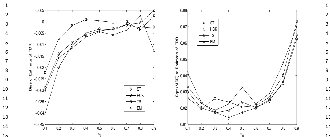
FIG 10. Bias and \sqrt{MSE} of \widehat{FDR} for ST, HCK, TS and EM Estimators for Beta Model (Data Generated by Normal Model)
