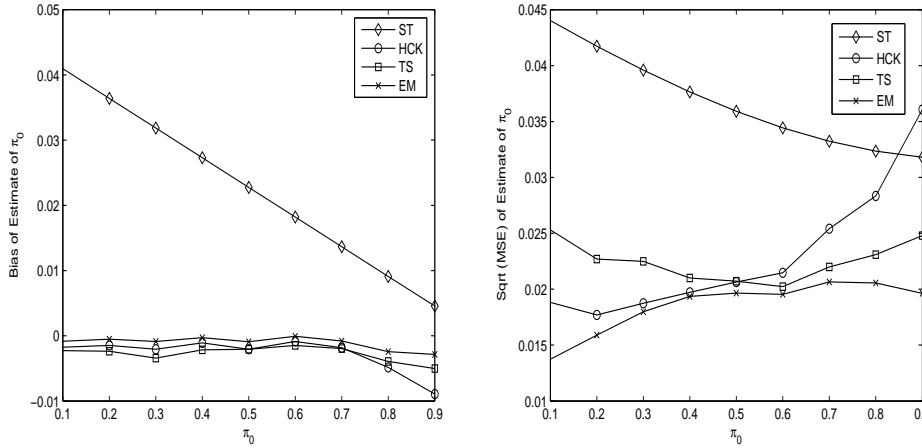
FIG 1. Bias and \sqrt{MSE} of \hat{\pi}_0 for ST, HCK, TS and EM Estimators for Normal Model (Data Generated by Normal Model with Fixed \delta )
