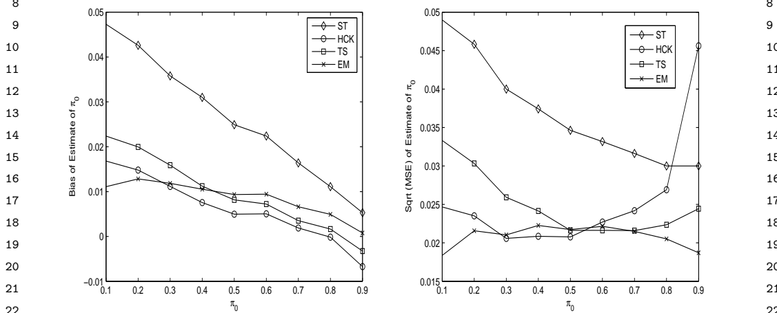
23 24 FIG 3. Bias and \sqrt{\text{MSE}} of \hat{\pi}_0 for ST, HCK, TS and EM Estimators for Normal Model (Data 25 Generated by Normal Model with Random \delta ) 26
