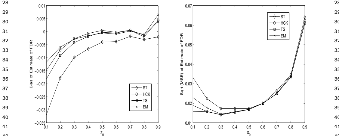
27 28 29 30 31 32 33 34 35 36 37 38 39 40 41 42 43 44 FIG 4. Bias and \sqrt{\text{MSE}} of \widehat{\text{FDR}} for ST, HCK, TS and EM Estimators for Normal Model (Data 45 Generated by Normal Model with Random \delta ) 46
