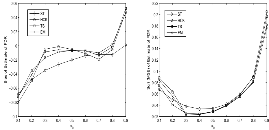
FIG 6. Bias and \sqrt{MSE} of \hat{FDR} for ST, HCK, TS and EM Estimators for Normal Model (Data Generated by Beta Model)
