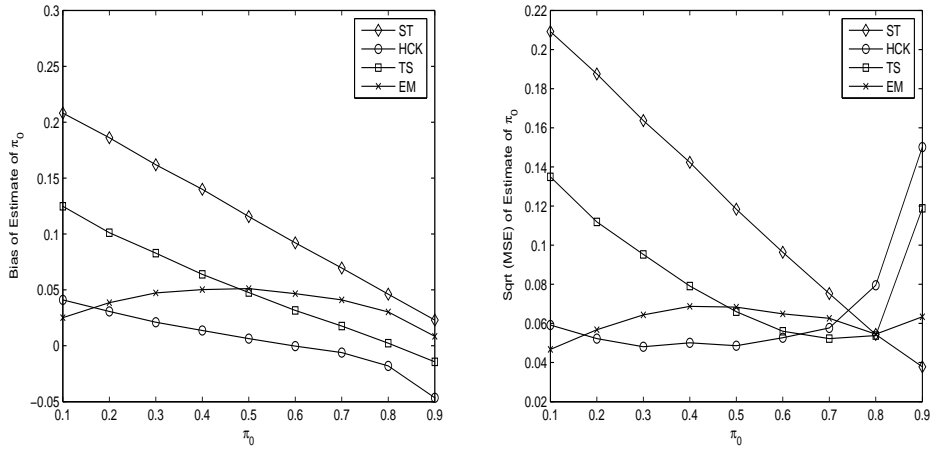
FIG 5. Bias and \sqrt{MSE} of \hat{\pi}_0 for ST, HCK, TS and EM Estimators for Normal Model (Data Generated by Beta Model)
