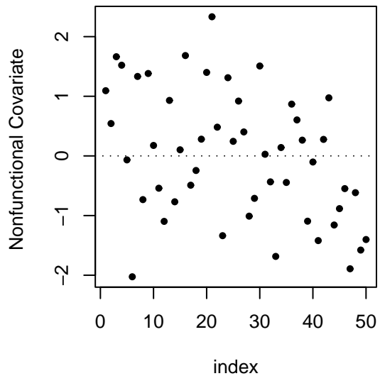
Simulated Data--Nonfunctional Covariate
