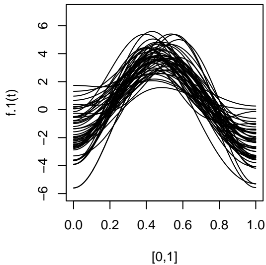
Simulated Data--Functional Covariate- 1
