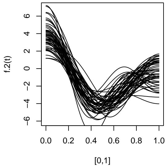
Simulated Data--Functional Covariate- 2
