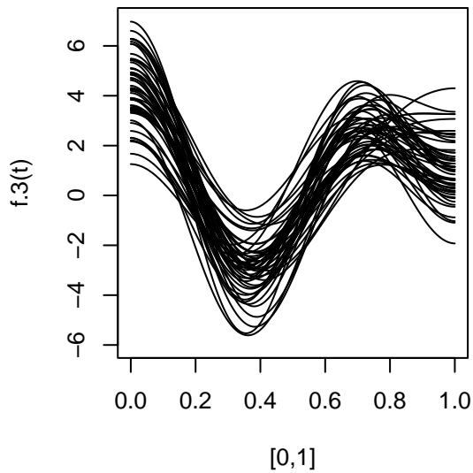
Simulated Data--Functional Covariate- 3
