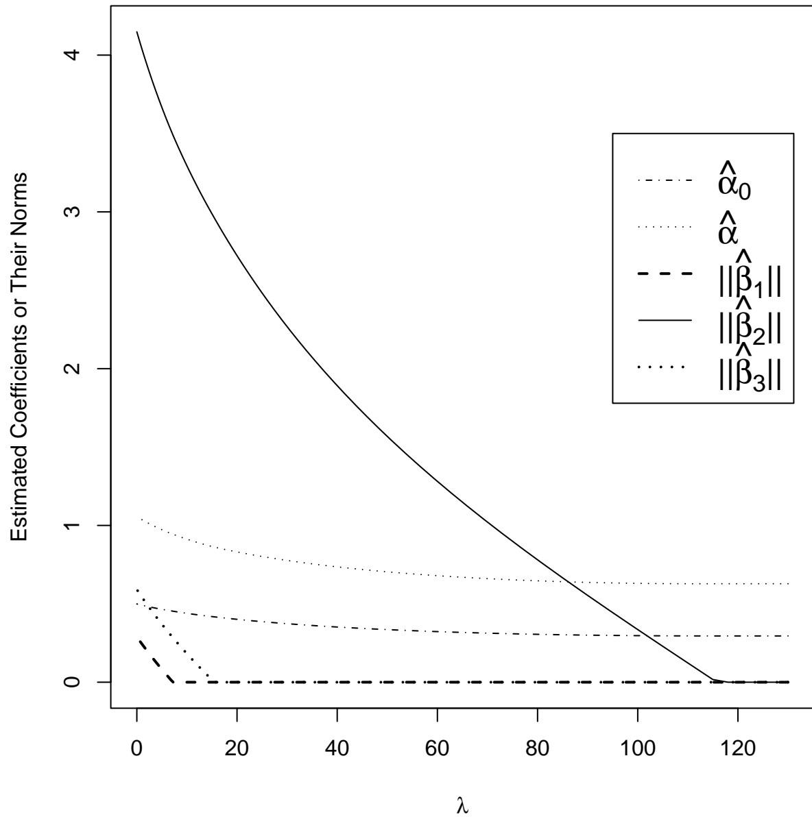
Coefficient Estimates v.s. \lambda
