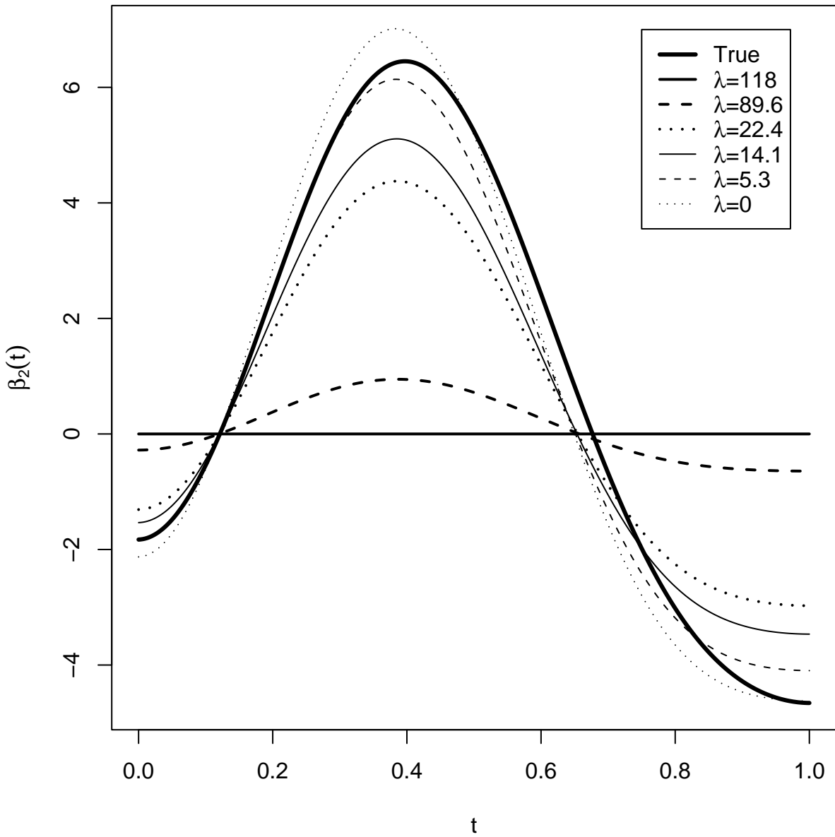
\hat{\beta}_2(t) at different \lambda
