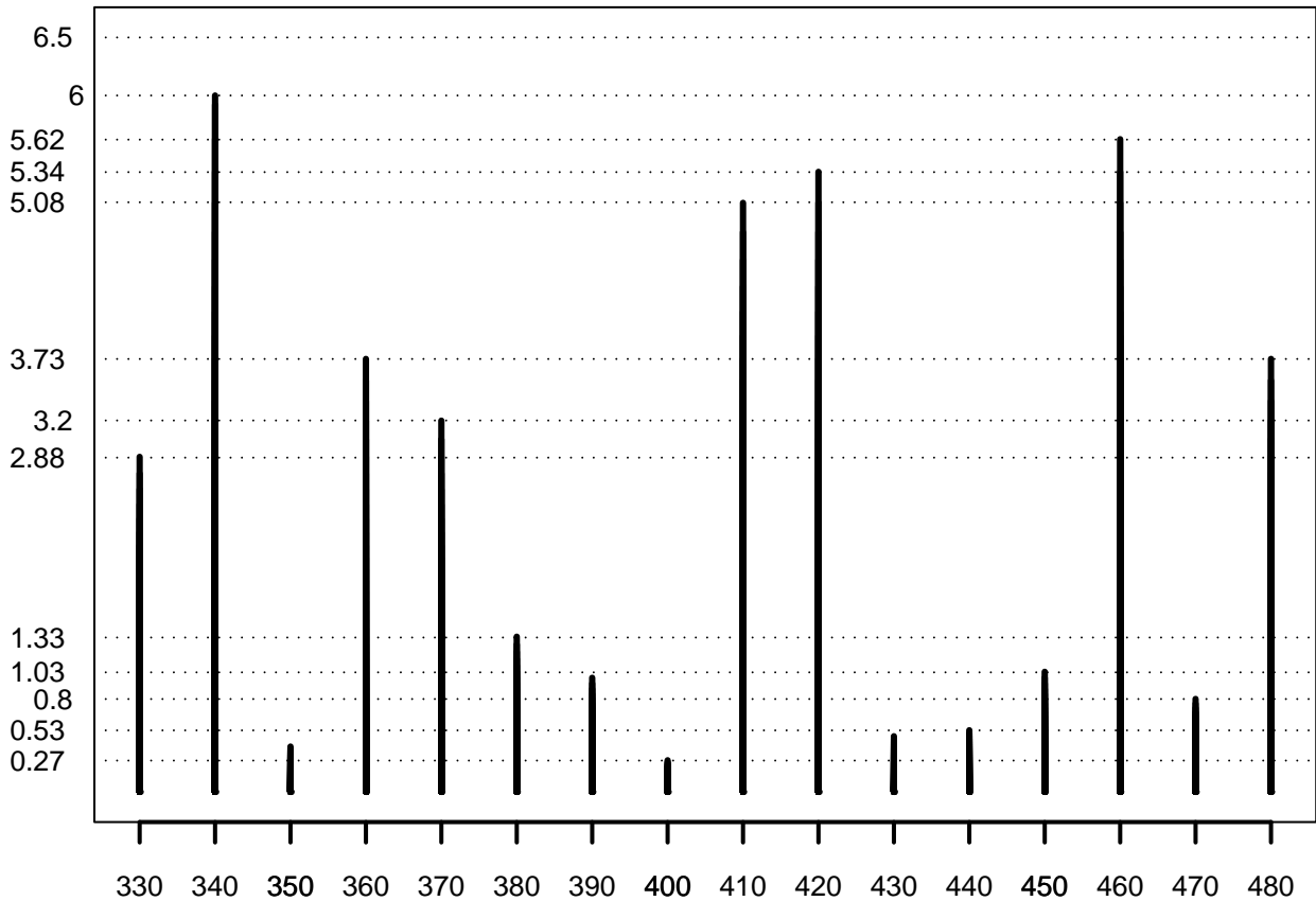
The selected functional predictors at different \lambda values
