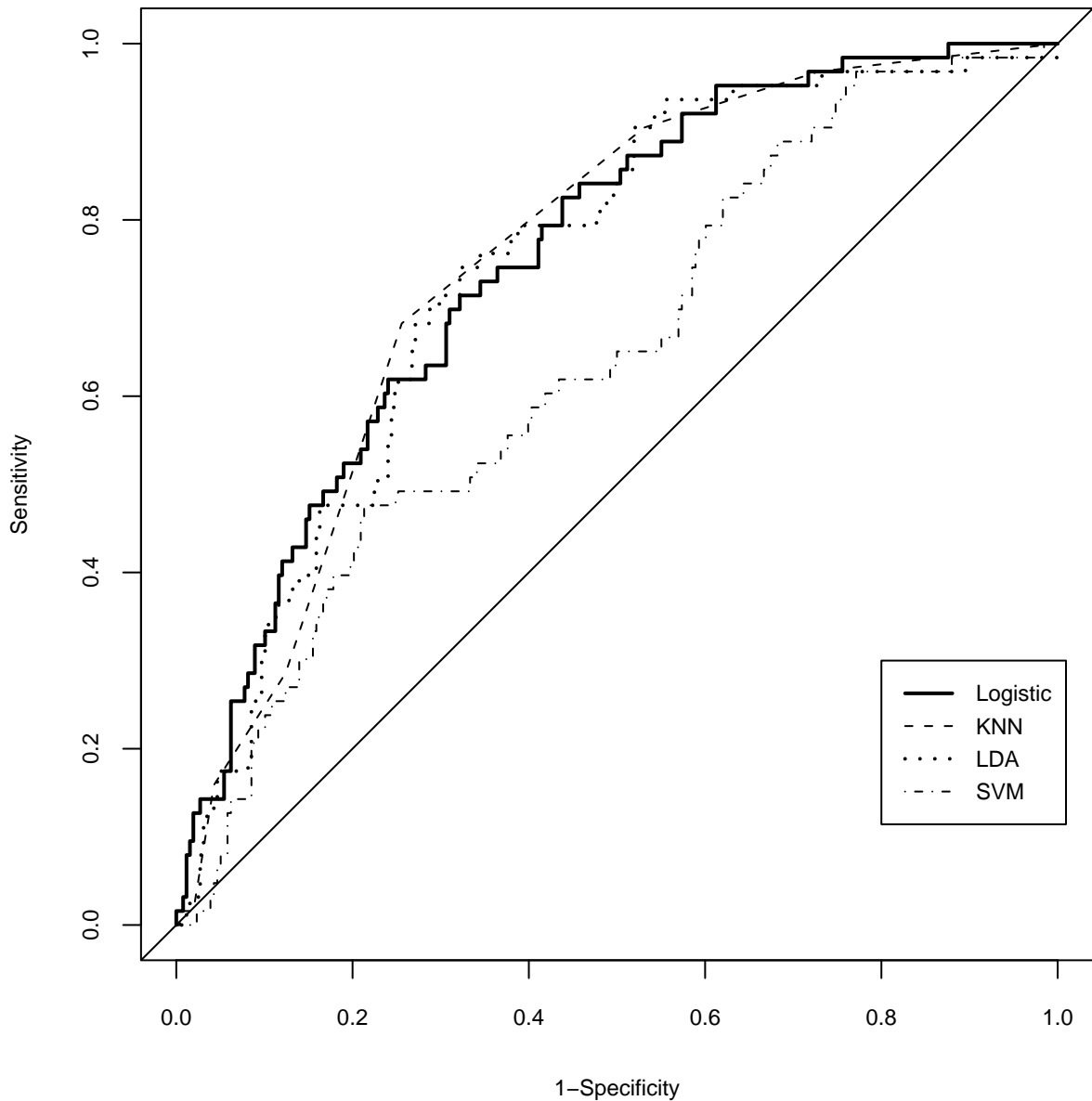
Empirical ROC curves for the test set prediction
