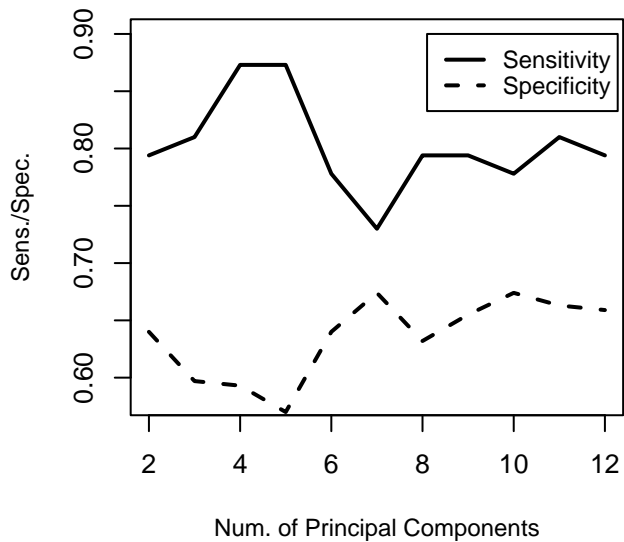
Sens. and Spec. vs. Num. of PC
