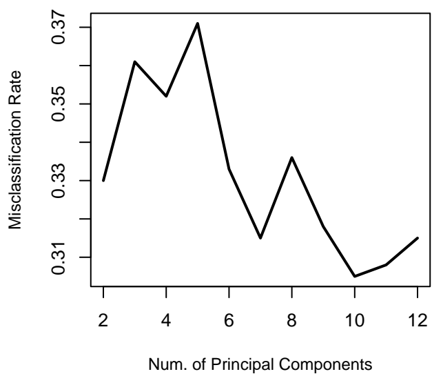
Misclassification Rate vs. Num. of PC
