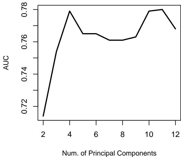
The Area Under ROC Curve vs. Num. of PC
