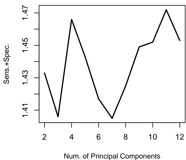
The Sum of Sens. and Spec. vs. Num. of PC
