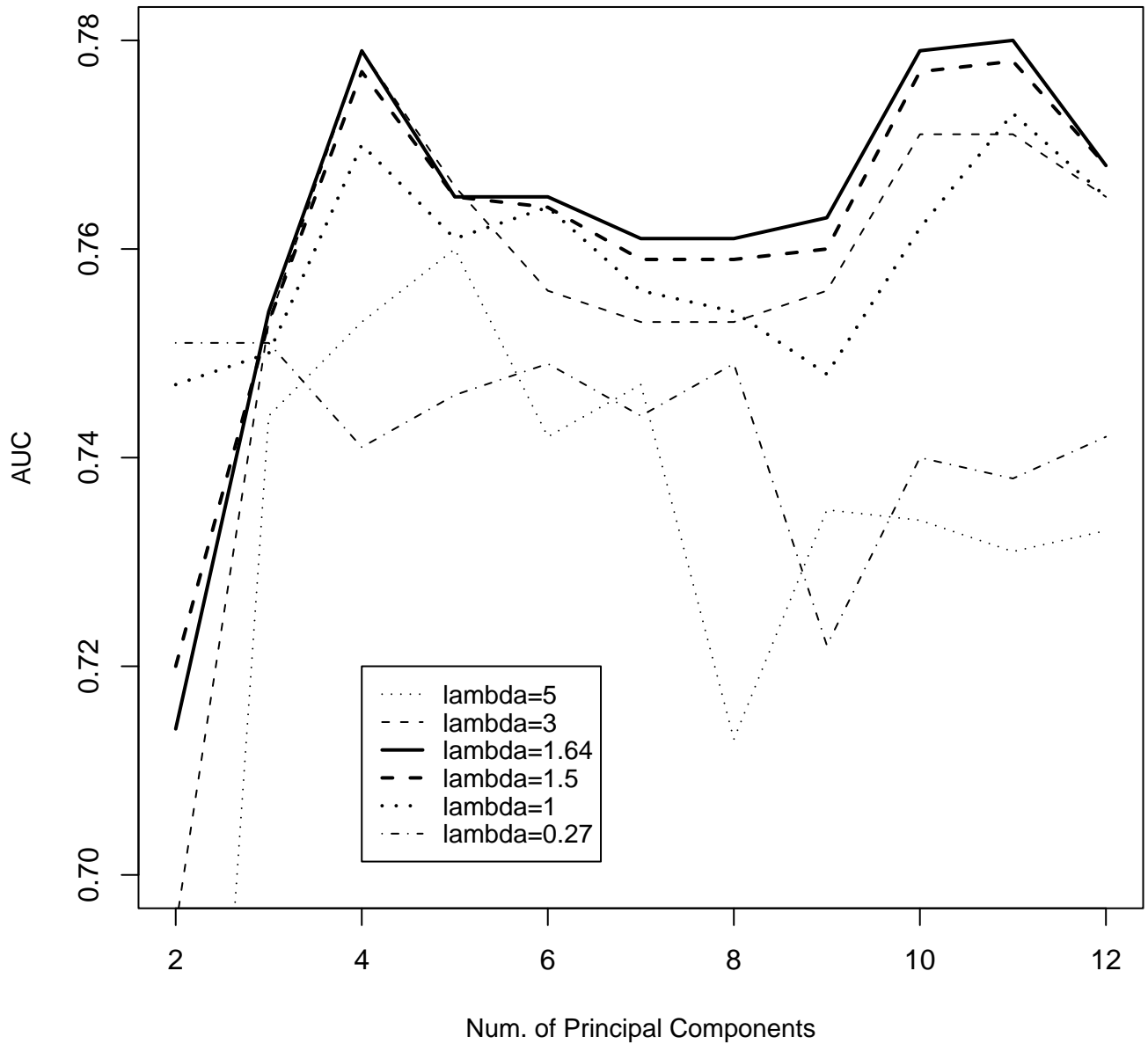
The Area Under ROC Curve v.s. Num. of PC
