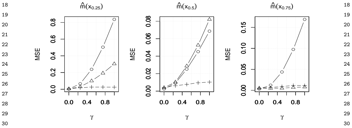
FIG 9. MSE of the three estimates of m(x) as a function of the misspecification parameter \gamma for (\lambda_1, \lambda_2, \alpha_1, \sigma^2) = (1, 1, 0.5, 1) . \circ = I , \triangle = II , + = III .
