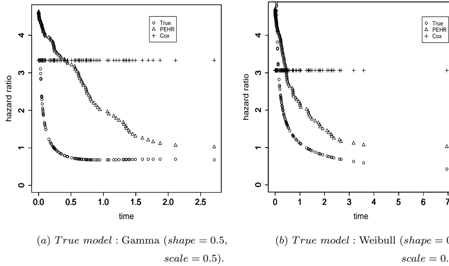
FIG 2. Cox and PEHR estimated hazard ratio when F_0 \sim EXP(1) and F \sim Gamma or Weibull.
