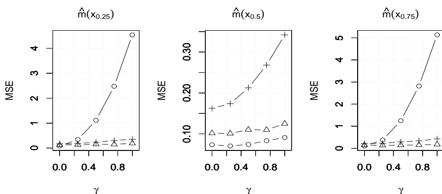
FIG 11. MSE of the three estimates of m(x) as a function of the misspecification parameter \gamma for (\lambda_1, \lambda_2, \alpha_1, \sigma^2) = (0.5, 0.5, 0.5, 1) . \circ = I , \triangle = II , + = III .
