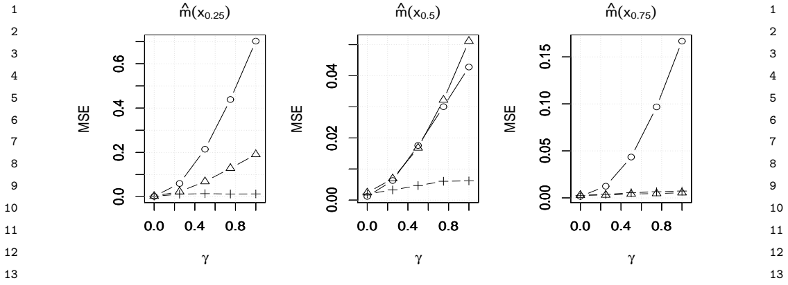
FIG 8. MSE of the three estimates of m(x) as a function of the misspecification parameter \gamma for (\lambda_1, \lambda_2, \alpha_1, \sigma^2) = (1, 1, 0.5, 0.5) . \circ = I , \triangle = II , + = III .
