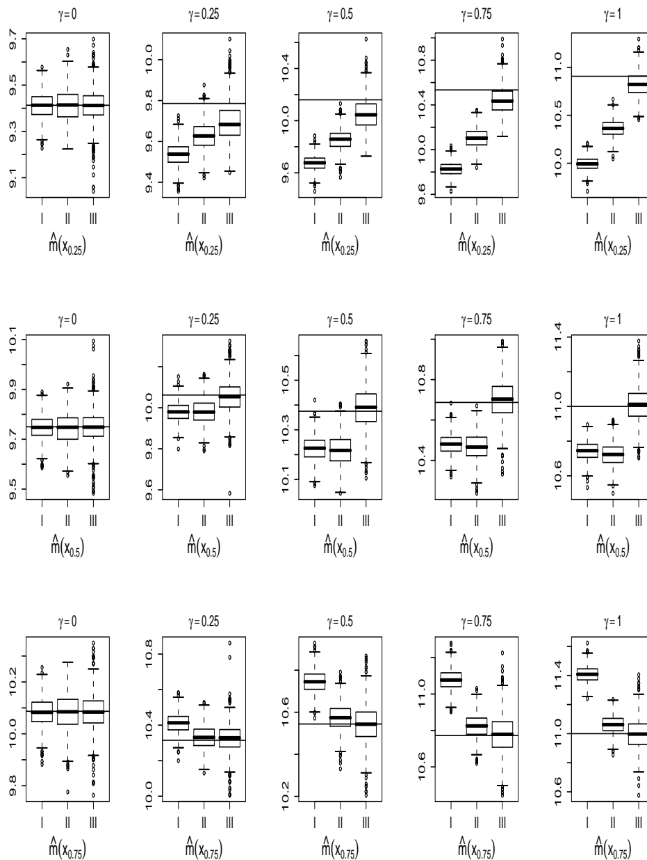
FIG 5. Boxplots of the three estimates of median regression m(x) for model (8.9) with (\lambda_1, \lambda_2, \alpha_1, \sigma^2) = (1, 1, 0.5, 1) . I: profile MLE, II: normal scores, and III: NP, spline. The true value of m(x) is the solid line.
