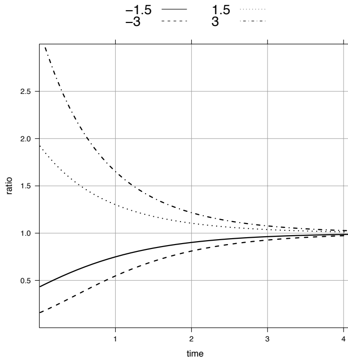
FIG 1. SINAMI and PEHR hazard ratios for \theta = -3, -1.5, 1.5, 3 .
