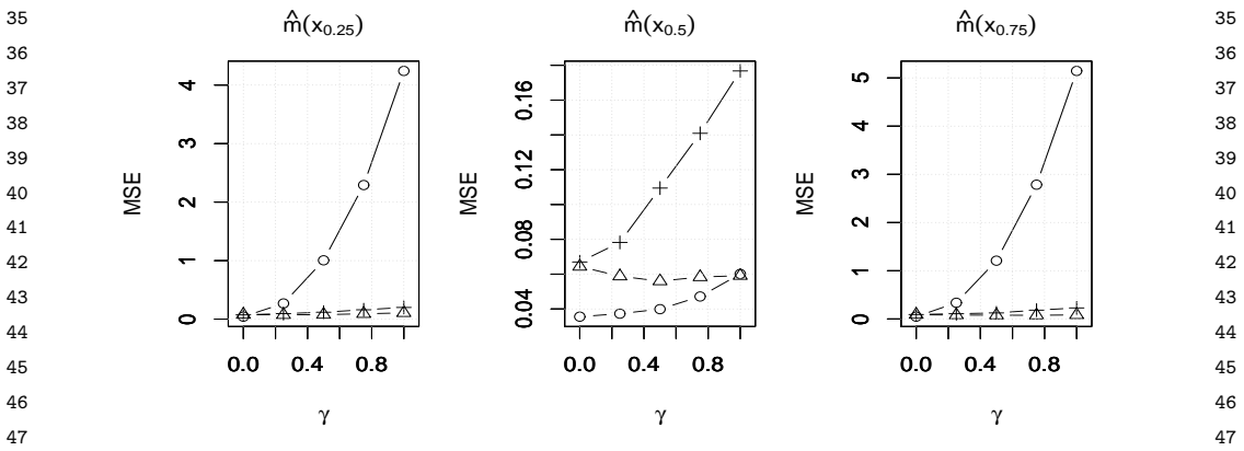
FIG 10. MSE of the three estimates of m(x) as a function of the misspecification parameter \gamma for (\lambda_1, \lambda_2, \alpha_1, \sigma^2) = (0.5, 0.5, 0.5, 0.5) . \circ = I , \triangle = II , + = III .
